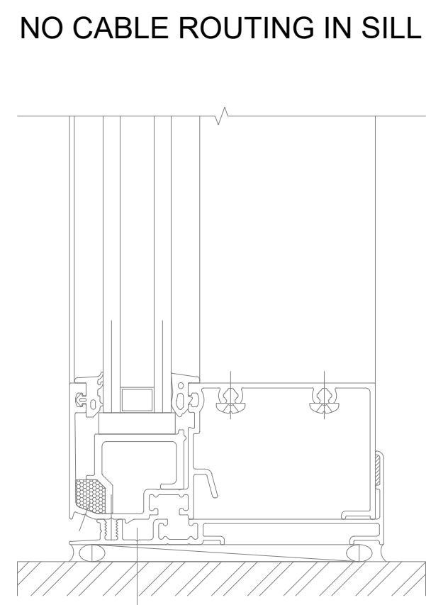
DETAIL 3 SILL
